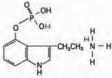
NORBAEOCYSTIN
